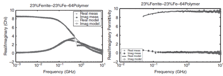
Figure 12.7 Data show measurements and fit to a two phase magnetic composite. Model and measurement have near overlaps.
